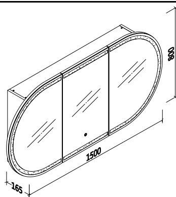
MC-PIAZA-150LED
