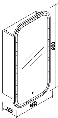
MC-PIAZA-45LED
