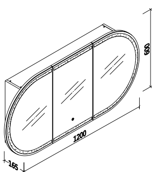
MC-PIAZA-120LED
